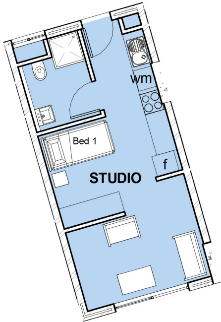
FLOOR PLAN - TYPE I1
